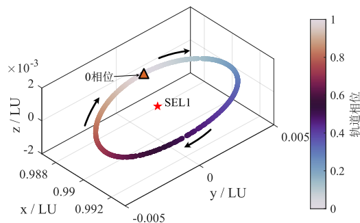
图6 Halo 相位定义 (S-B1 旋转系) Fig.6 Halo phase definition (S-B1 rotating frame)
