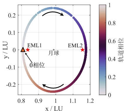
图5 DRO 相位定义 (E-M 旋转系) Fig.5 DRO phase definition (E-M rotating frame)
